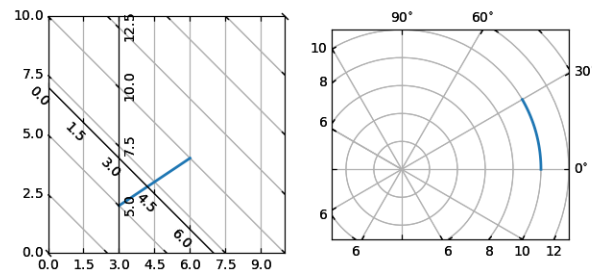
Fig. 77: Demo Curvelinear Grid
