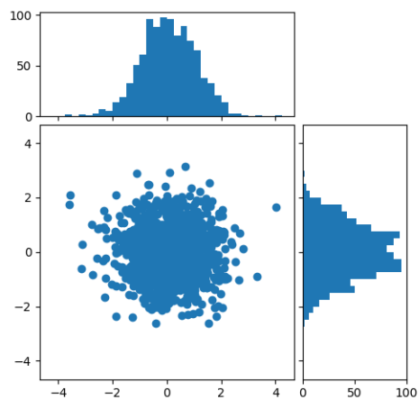
Fig. 83: Scatter Hist
