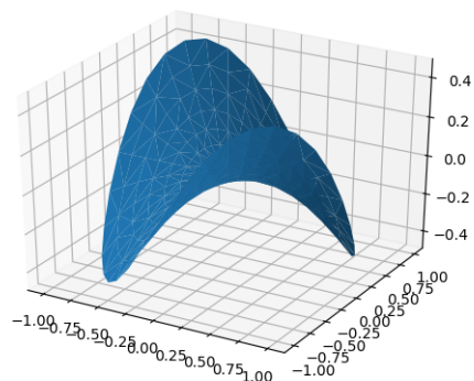
Fig. 52: Trisurf3d
